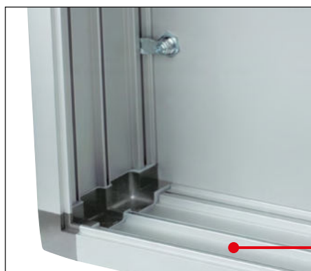
All-round mounting grooves simplify installation
